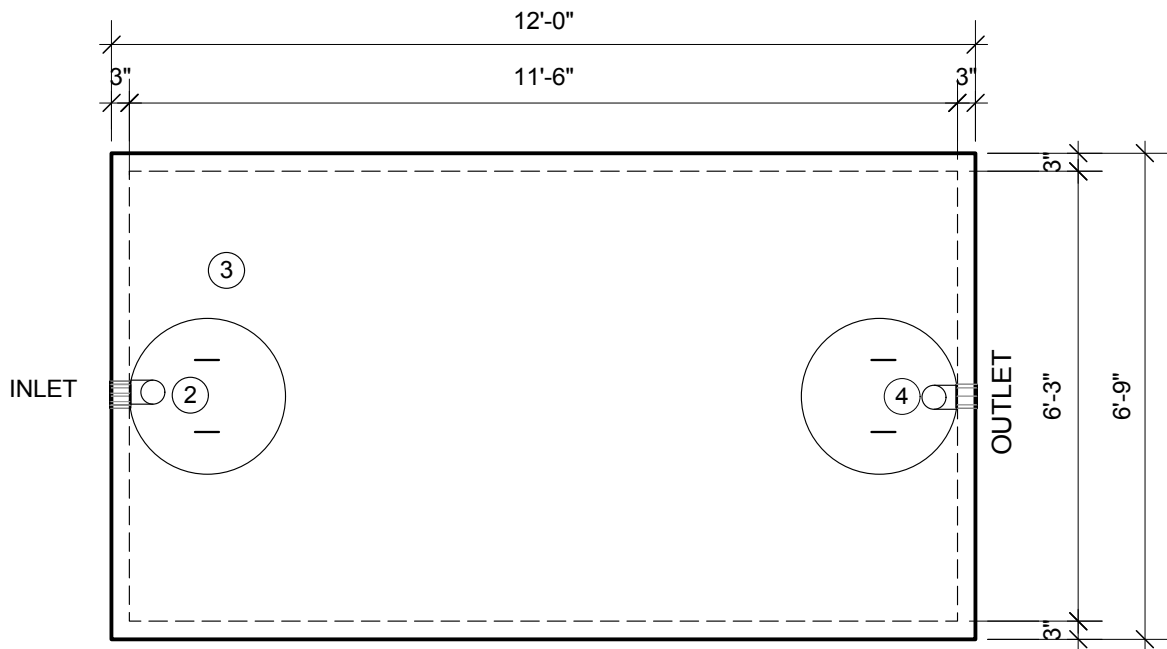
PLAN VIEW
